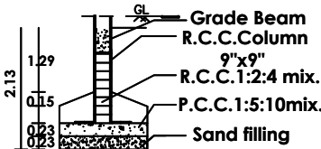
COLUMN DETAILS
