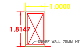
WICKET GATE
