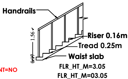
STAIRCASE DETAILS
