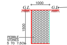
SECTION OF PEBBLE TRENCH
