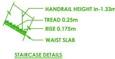
STAIRCASE DETAILS
