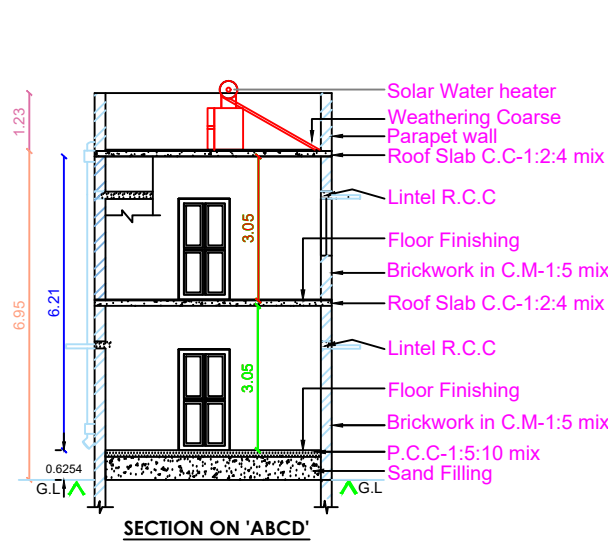
SECTION ON 'ABCD'
