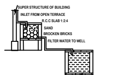
RAINWATER HARVESTING
