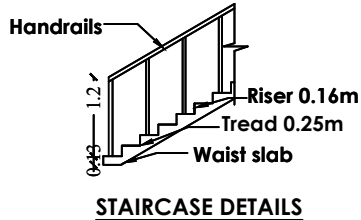
STAIRCASE DETAILS
