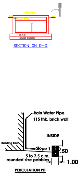
PERCOLATION PIT
