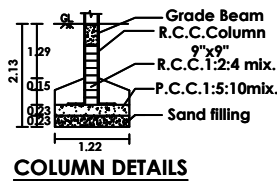
COLUMN DETAILS
