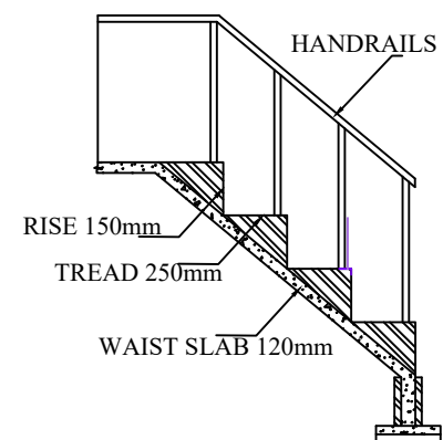
STAIRCASE DETAILS
