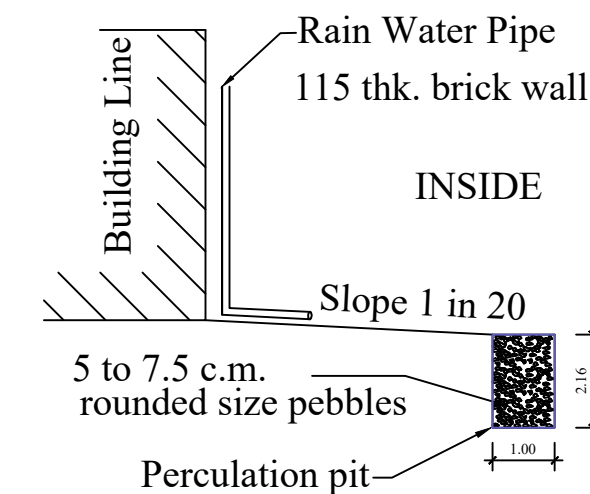
RAIN WATER HARVESTING PERCOLATION PIT
