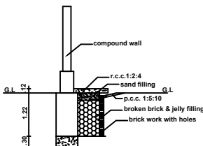
PLINTH BOUNDARY PERCOLATION PIT
