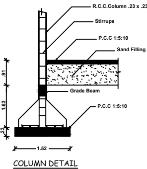
COLUMN DETAIL
