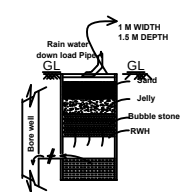
SEC. RAIN WATER HARVEST PIT
