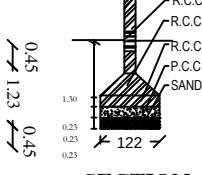
SECTION
