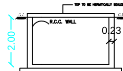
RCC WALL SECTION (SAMPLE) (RCC CAPACITY 1.5000/1.25)
