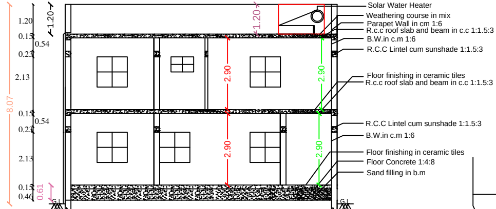
SECTION - "AB - CD "
