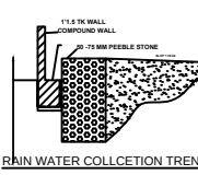
RAIN WATER COLLECTION TRENCH
