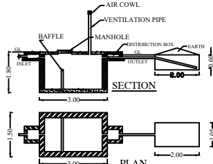
SEPTIC TANK DISPERSION TRENCH
