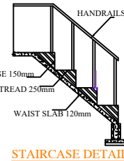
STAIRCASE DETAILS
