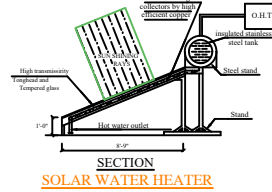
SECTION SOLAR WATER HEATER
