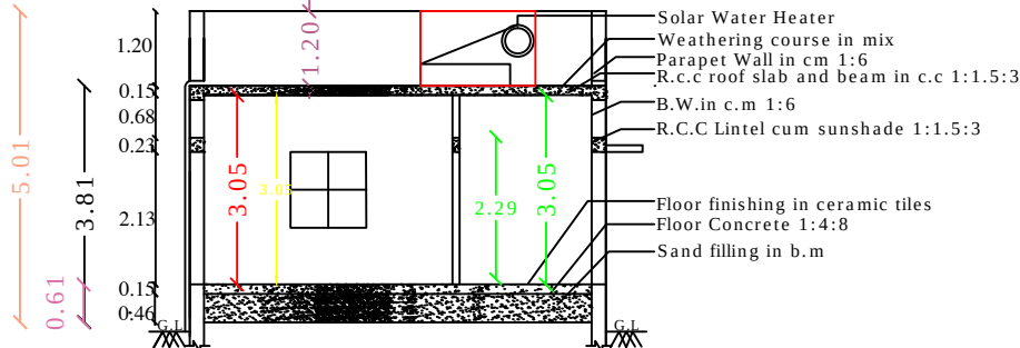
SECTION - "AB "
