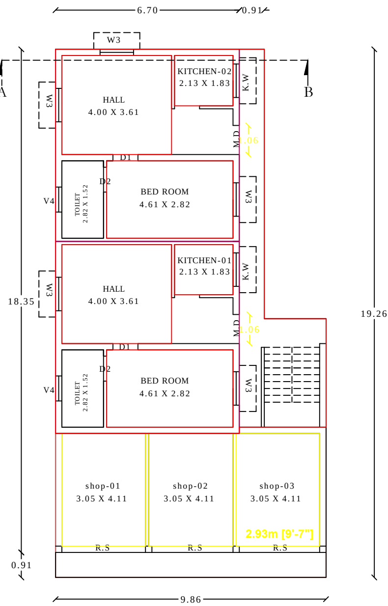
GROUND FLOOR
