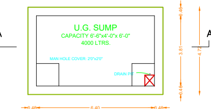
SUMP DETAIL
