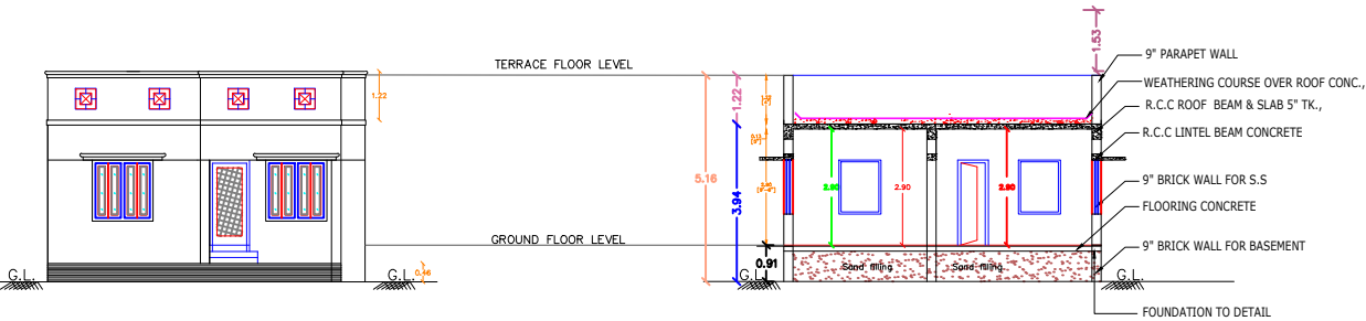
FRONT ELEVATION
