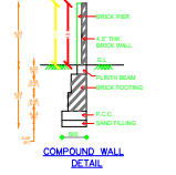
COMPOUNDING WALL DETAIL
