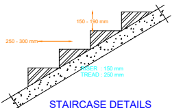
STAIRCASE DETAILS
