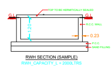
RWVH SECTION (SAMPLE)
