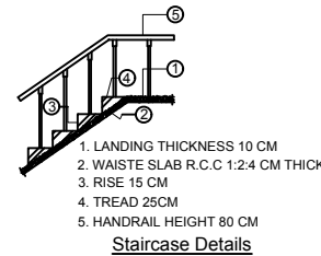
Staircase Details
