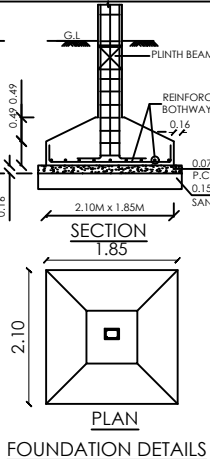
FOUNDATION DETAILS
