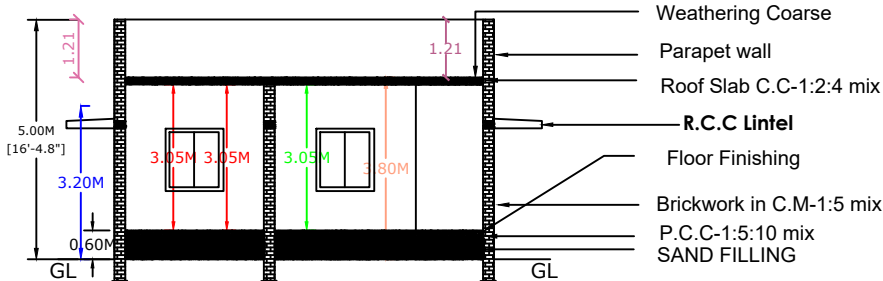
SECTION ON XX
