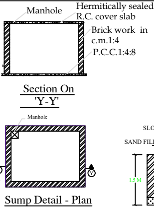
Sump Detail - Plan
