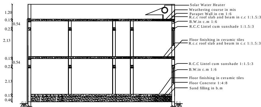
SECTION - "AB - CD "
