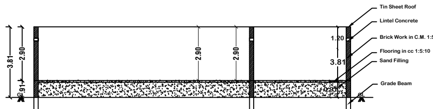
SECTION-AA
