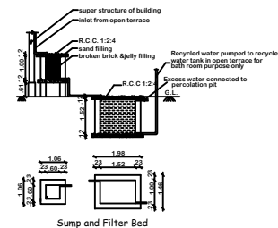
Sump and Filter Bed
