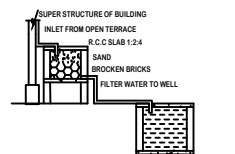
RAINWATER HARVESTING
