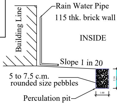
RAIN WATER HARVESTING PERCOLATION PIT RW_H_CAPACITY_L=2000LTRS
