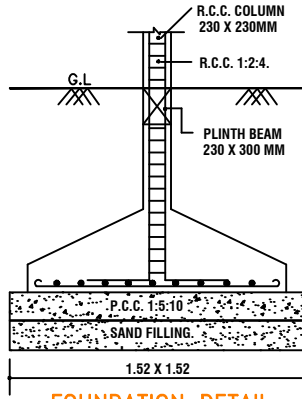
FOUNDATION DETAIL
