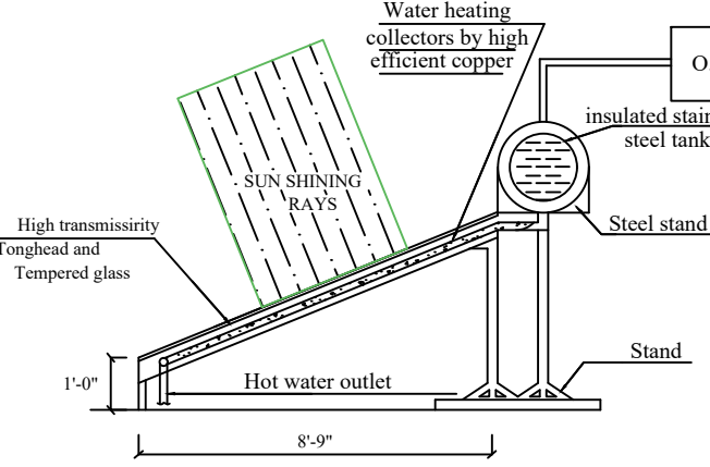
SECTION SOLAR WATER HEATER
