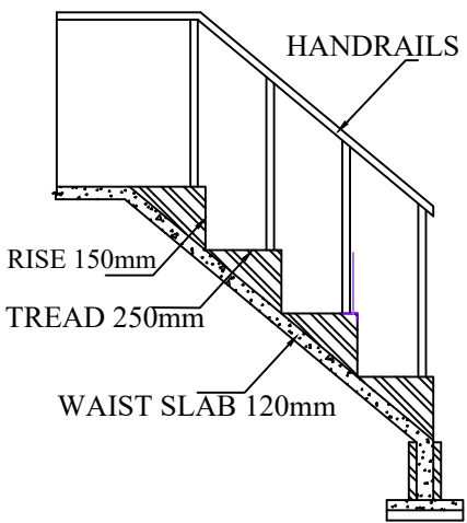
STAIRCASE DETAILS
