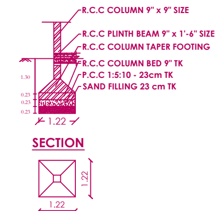
COLUMN DETAILS PLAN
