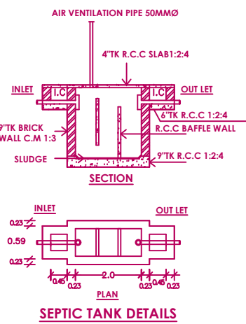
SEPTIC TANK DETAILS
