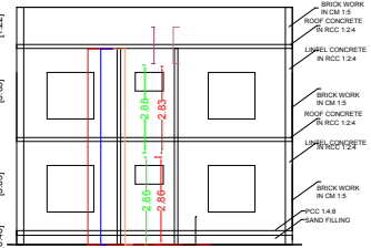
SECTION ON KR
