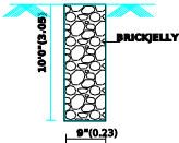
PERCOLATION PIT
