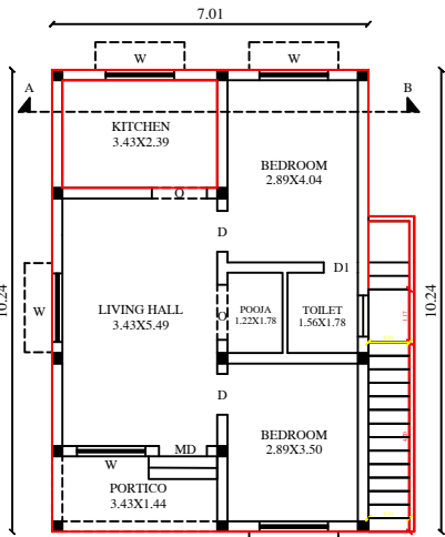
EXL. GROUND FLOOR PLAN
