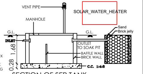
SECTION OF SEP.TANK
