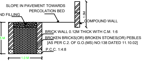
SECTION OF RAIN WATER PERCOLATION BED
