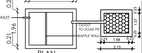
PLAN SEPTIC. TANK
