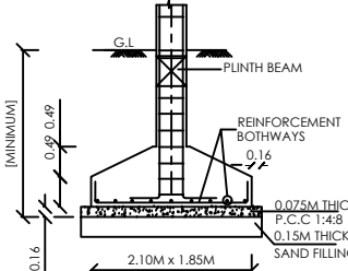
SECTION 1.85
