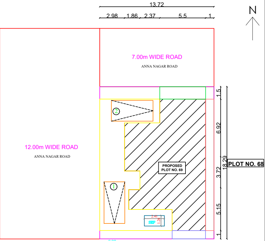
SITE PLAN
