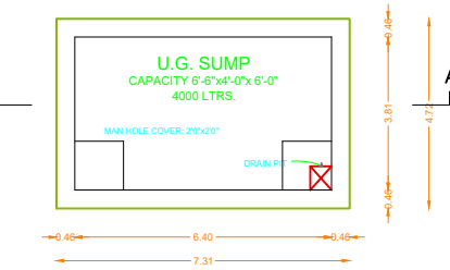
SUMP DETAIL
