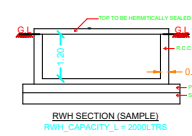
RWHT SECTION (SAMPLE)
