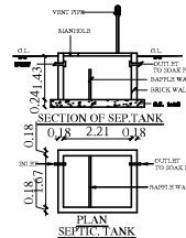
PLAN SEPTIC TANK
