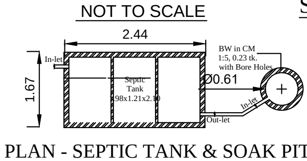
PLAN - SEPTIC TANK & SOAK PIT
