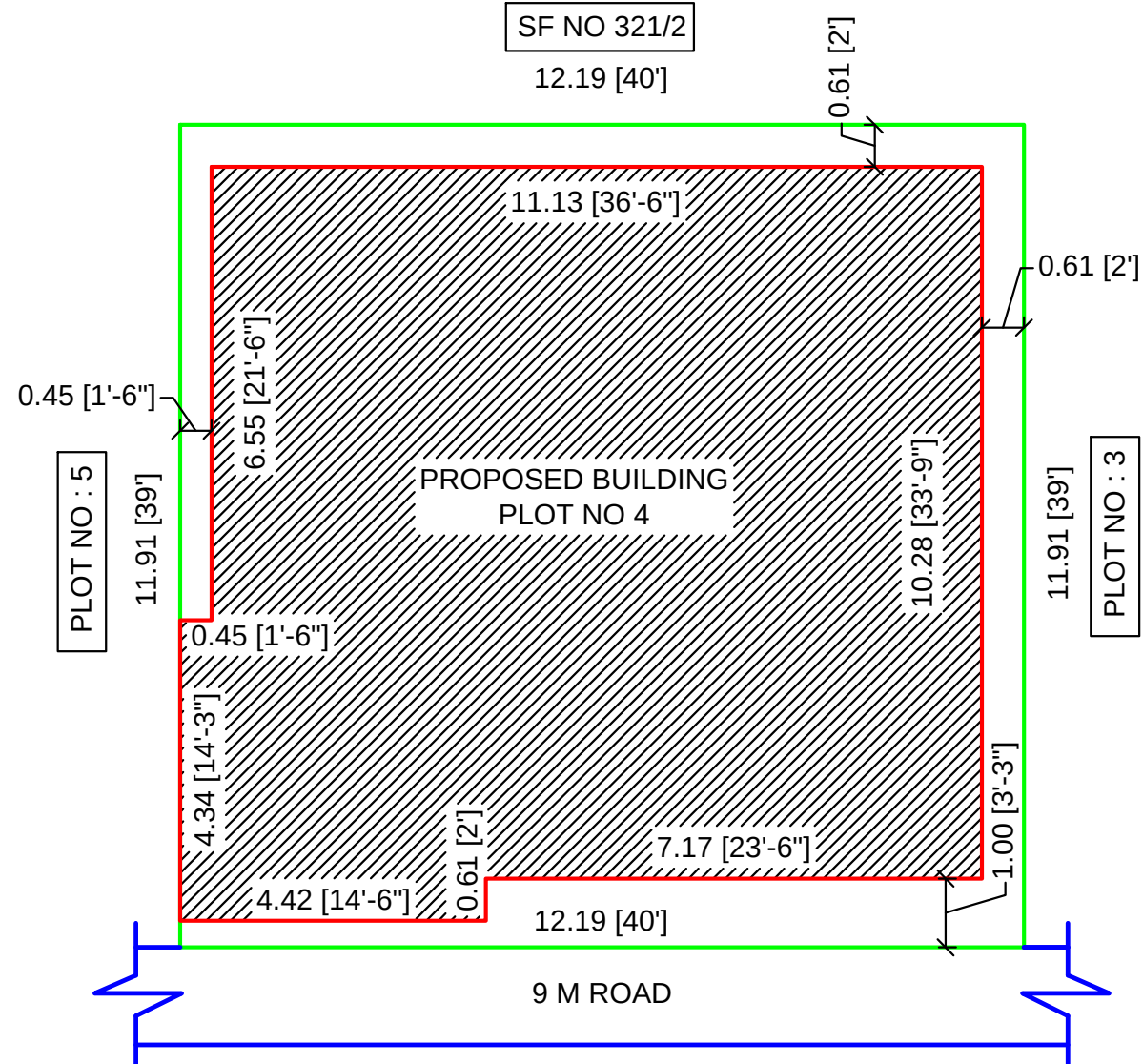
SITE PLAN (1:100)
