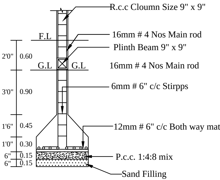
COLUMN DETIAL
