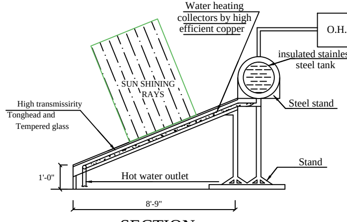
SECTION SOLAR WATER HEATER
