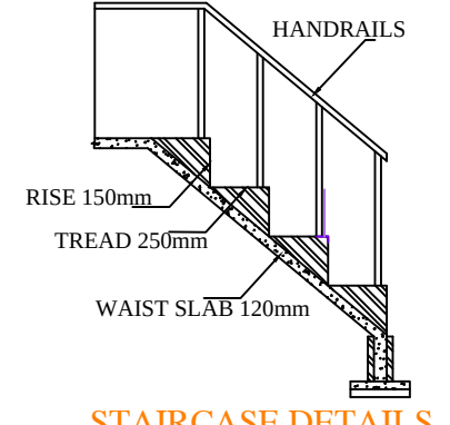
STAIRCASE DETAILS
