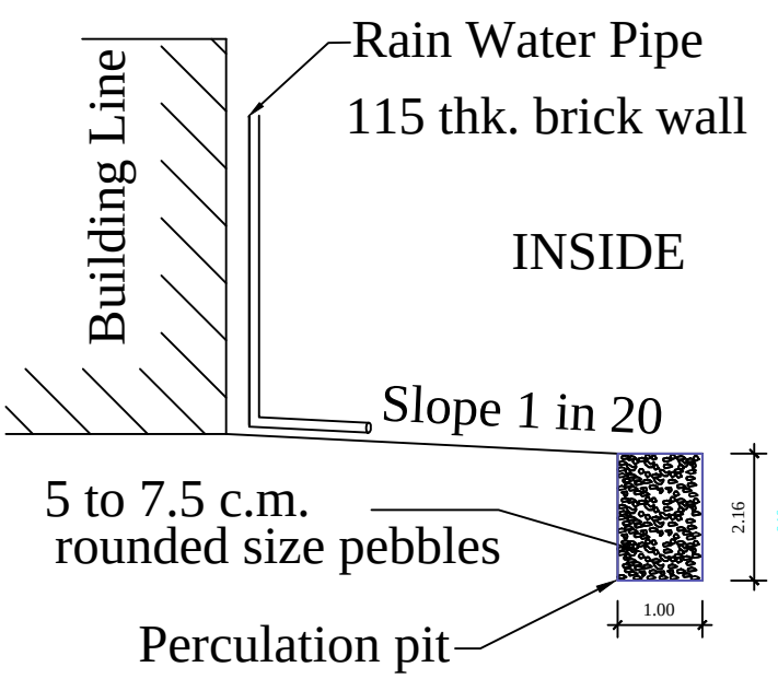
RAIN WATER HARVESTING PERCOLATION PIT RWH_CAPACITY_L=2000LTRS
