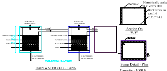
RAIN WATER COLL. TANK
