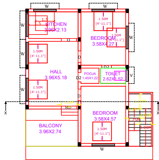
PRO.FIRST FLOOR PLAN
