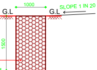
SECTION OF PEBBLE TRENCH SCALE : 1 : 100
