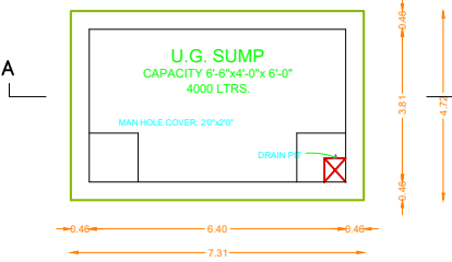
SUMP DETAIL
