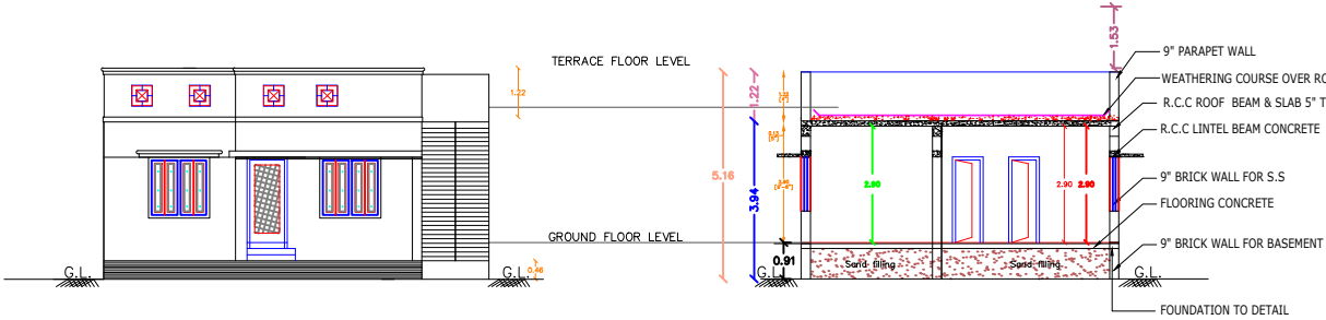
FRONT ELEVATION
