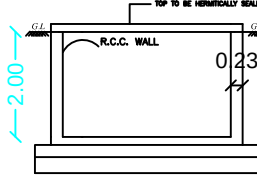
RWH SECTION (SAMPLE)
