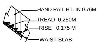
HAND RAIL HT. IN 0.76M
