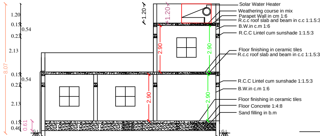
SECTION - "AB - CD "
