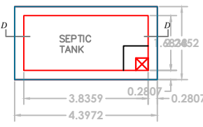
PLAN OF SEPTIC TANK SCALE 1"=2'0"
