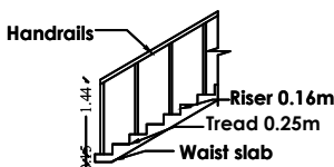
STAIRCASE DETAILS
