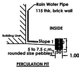
PERCOLATION PIT
