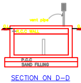
SECTION ON D-D
