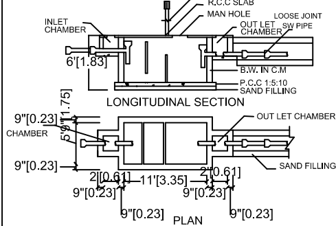
SEPTIC TANK:
