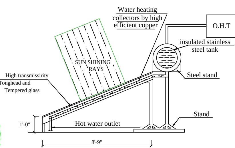
SECTION SOLAR WATER HEATER
