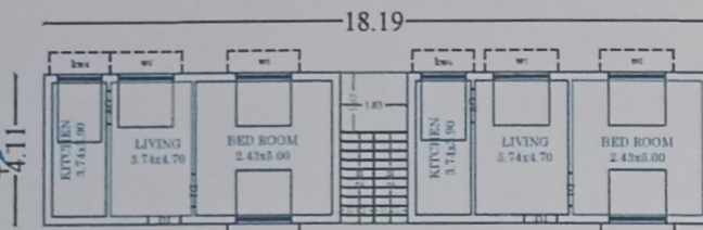
BLOCK I GROUND FLOOR PLAN
