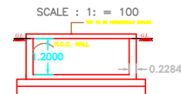
RW_SECTION (SAMPLE)
