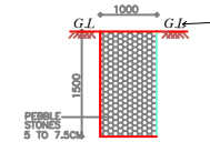
SECTION OF PEBBLE TRENCH
