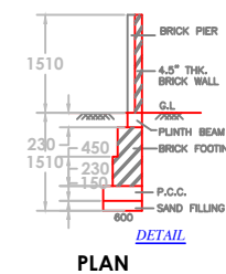
DETAIL
