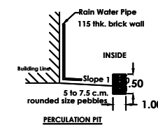
PERCOLATION PIT
