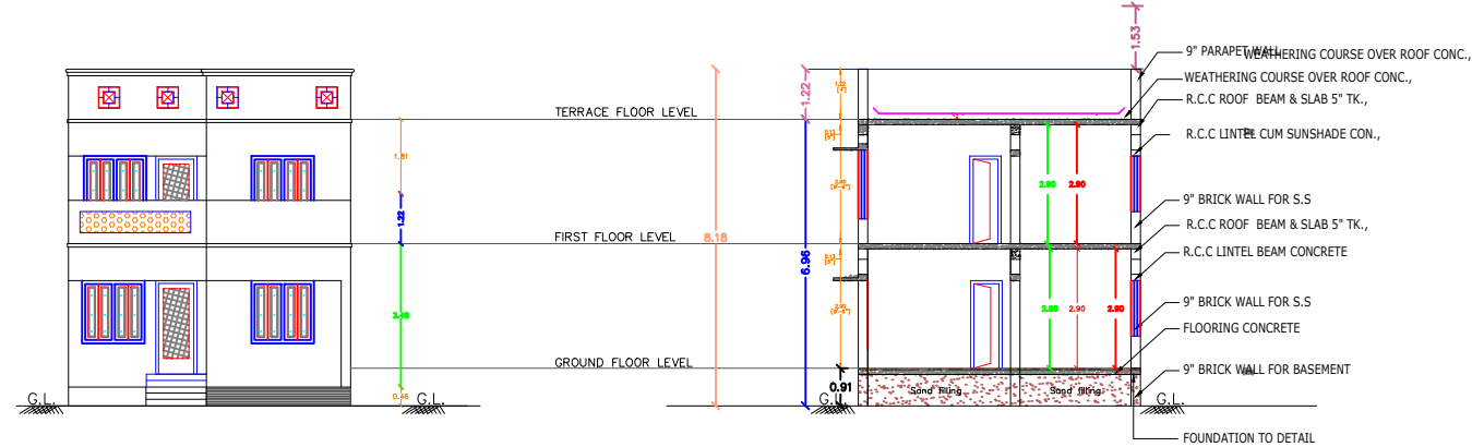
FRONT ELEVATION
