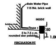
PERCOLATION PIT
