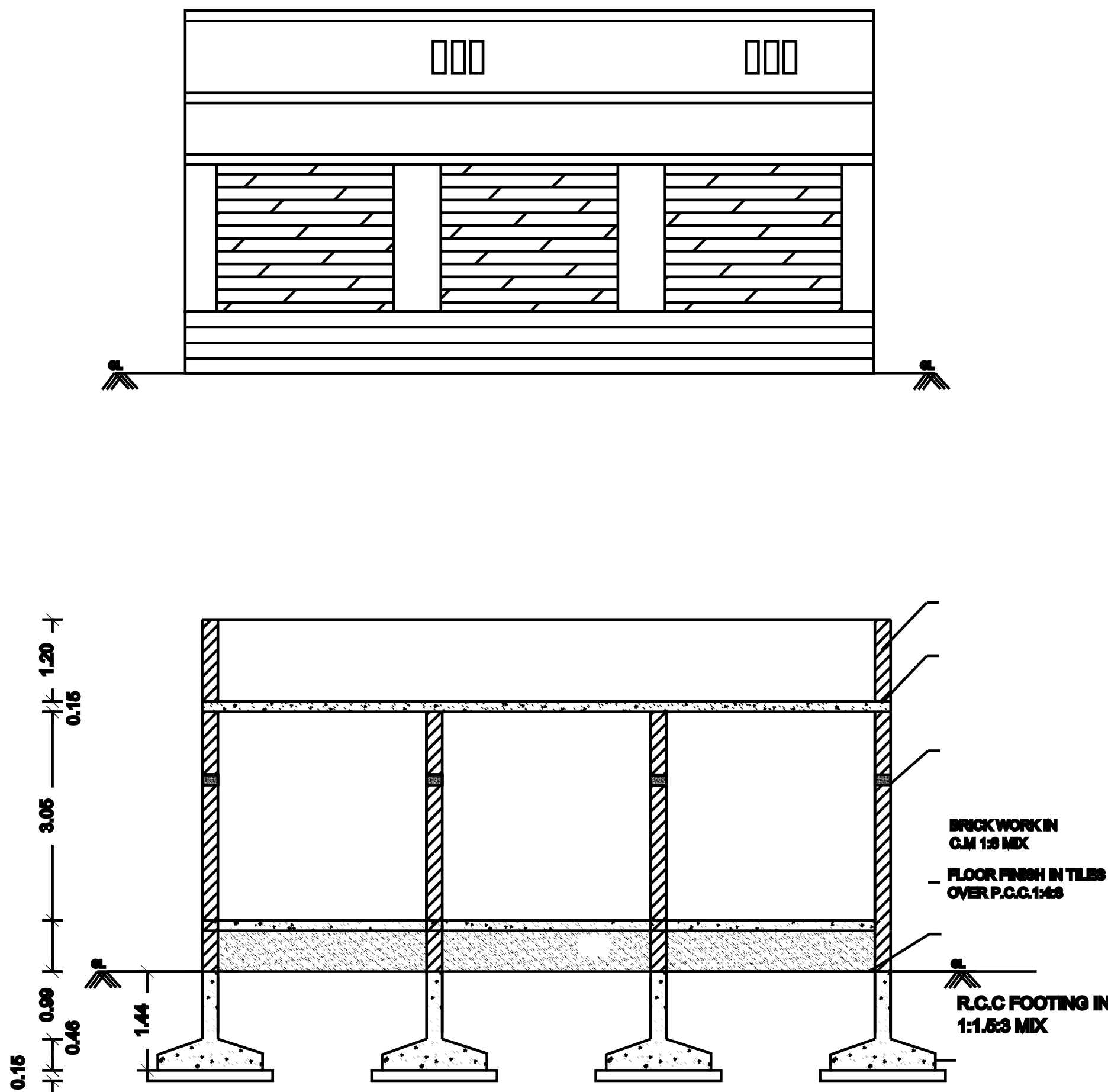
SECTION AA
