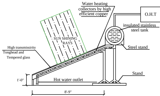
SECTION SOLAR WATER HEATER
