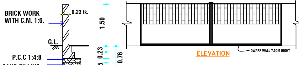
SECTION OF COMPOUND WALL
