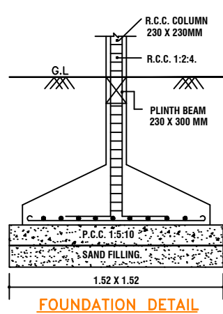
FOUNDATION DETAIL
