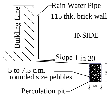
RAIN WATER HARVESTING PERCOLATION PIT RWH_CAPACITY_L=2000LTRS
