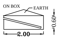
SECTION SOLAR WATER HEATER
