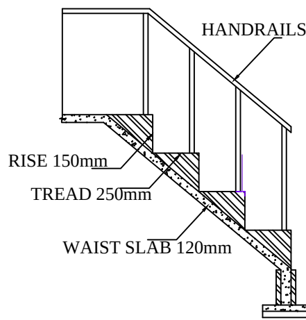
STAIRCASE DETAILS
