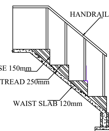
STAIRCASE DETAILS
