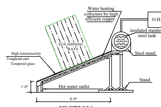
SECTION SOLAR WATER HEATER
