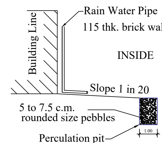
RAIN WATER HARVESTING PERCOLATION PIT RW_H_CAPACITY_L=2000LTRS
