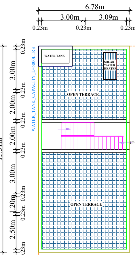
TERRACE PLAN
