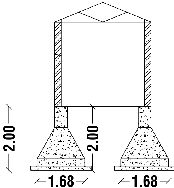
SECTION - "AB "
