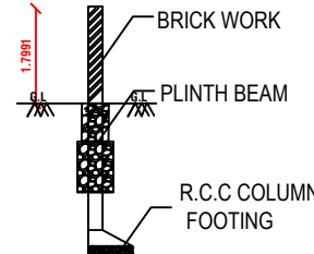
SECTION
