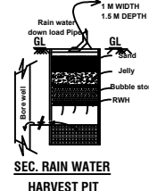
SEC. RAIN WATER HARVEST PIT
