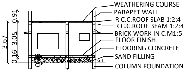
SECTION- SS
