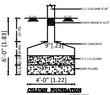
COLUMN FOUNDATION
