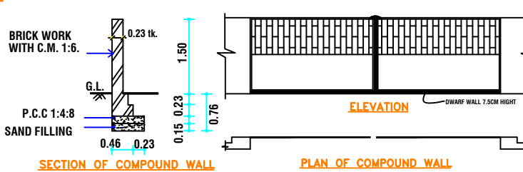
SECTION OF COMPOUND WALL
