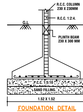
FOUNDATION DETAIL
