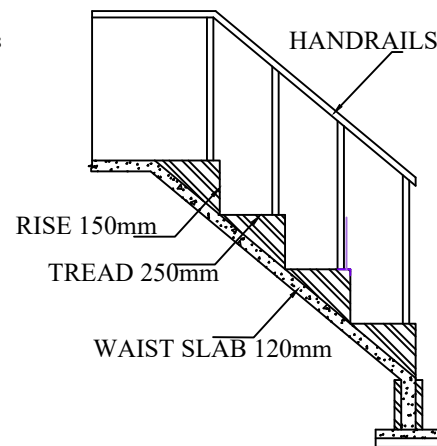
STAIRCASE DETAILS
