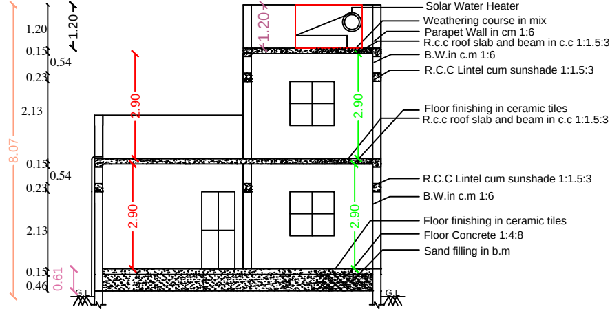
SECTION - "AB "
