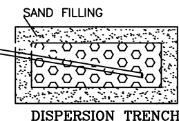
DISPERSION TRENCH
