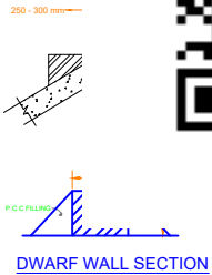
DWARF WALL SECTION NOT TO SCALE
