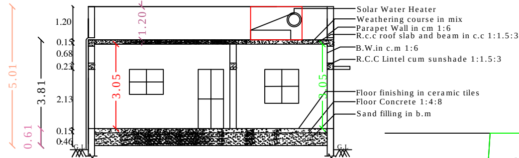
SECTION - "AB "
