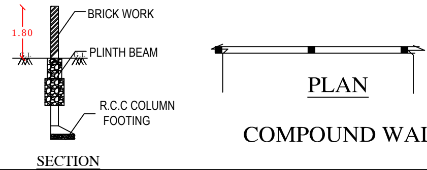
SECTION
