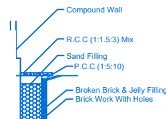
WATER HARVEST DETAILS
