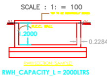
SECTION OF SEPTIC TANK
