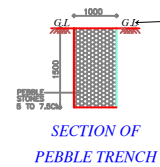
SECTION OF PEBBLE TRENCH
