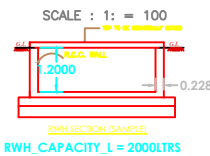
SECTION OF MAIN GATE
